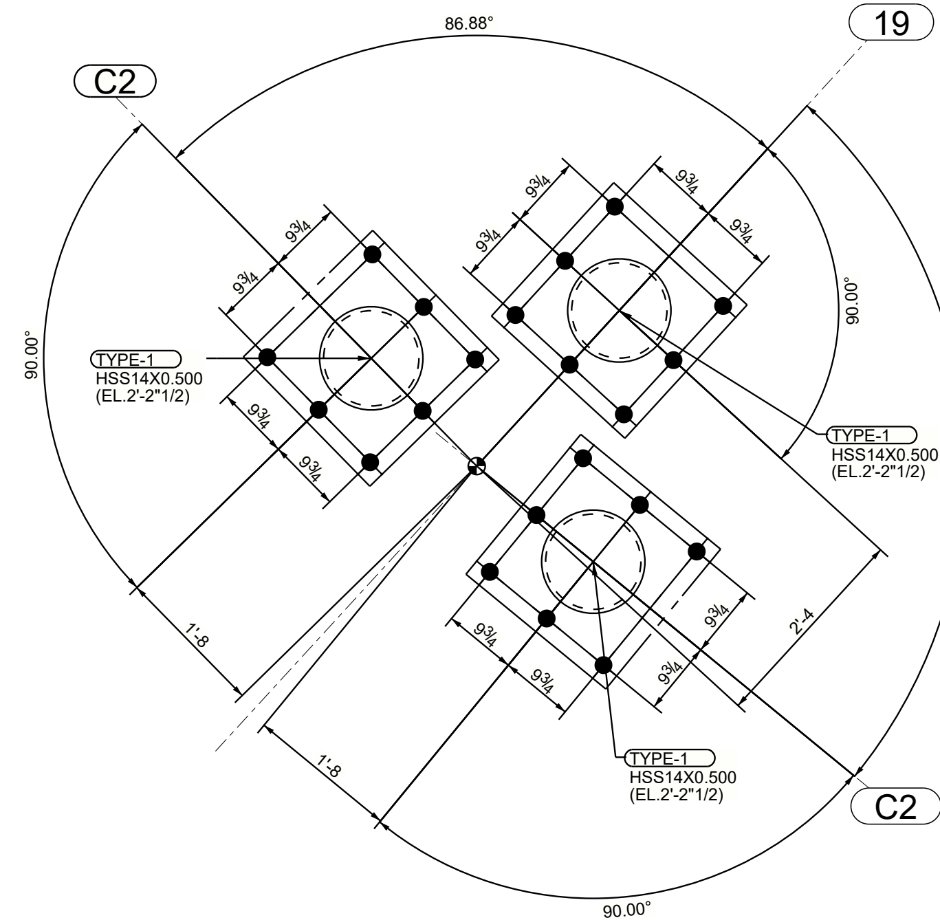
DETAIL C 1-A102
