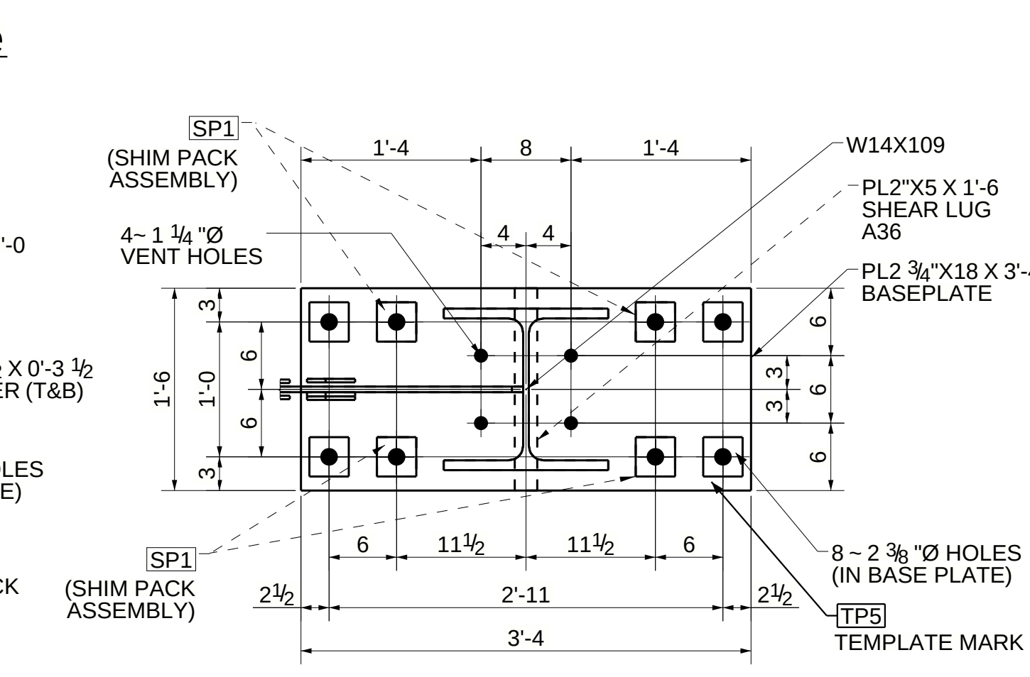
TYPE-5 (08 LOCATIONS)
