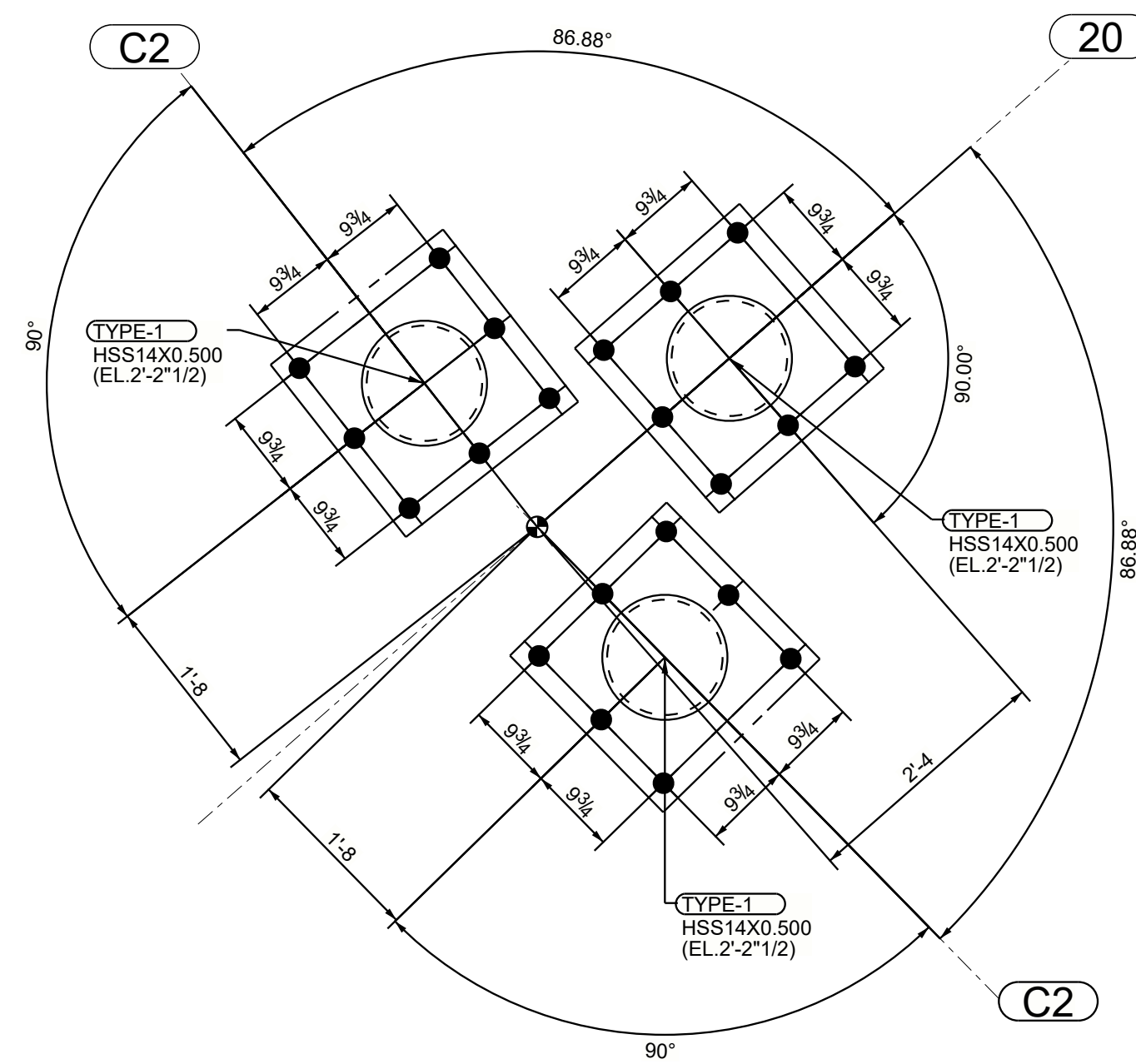
DETAIL B 1-A102
