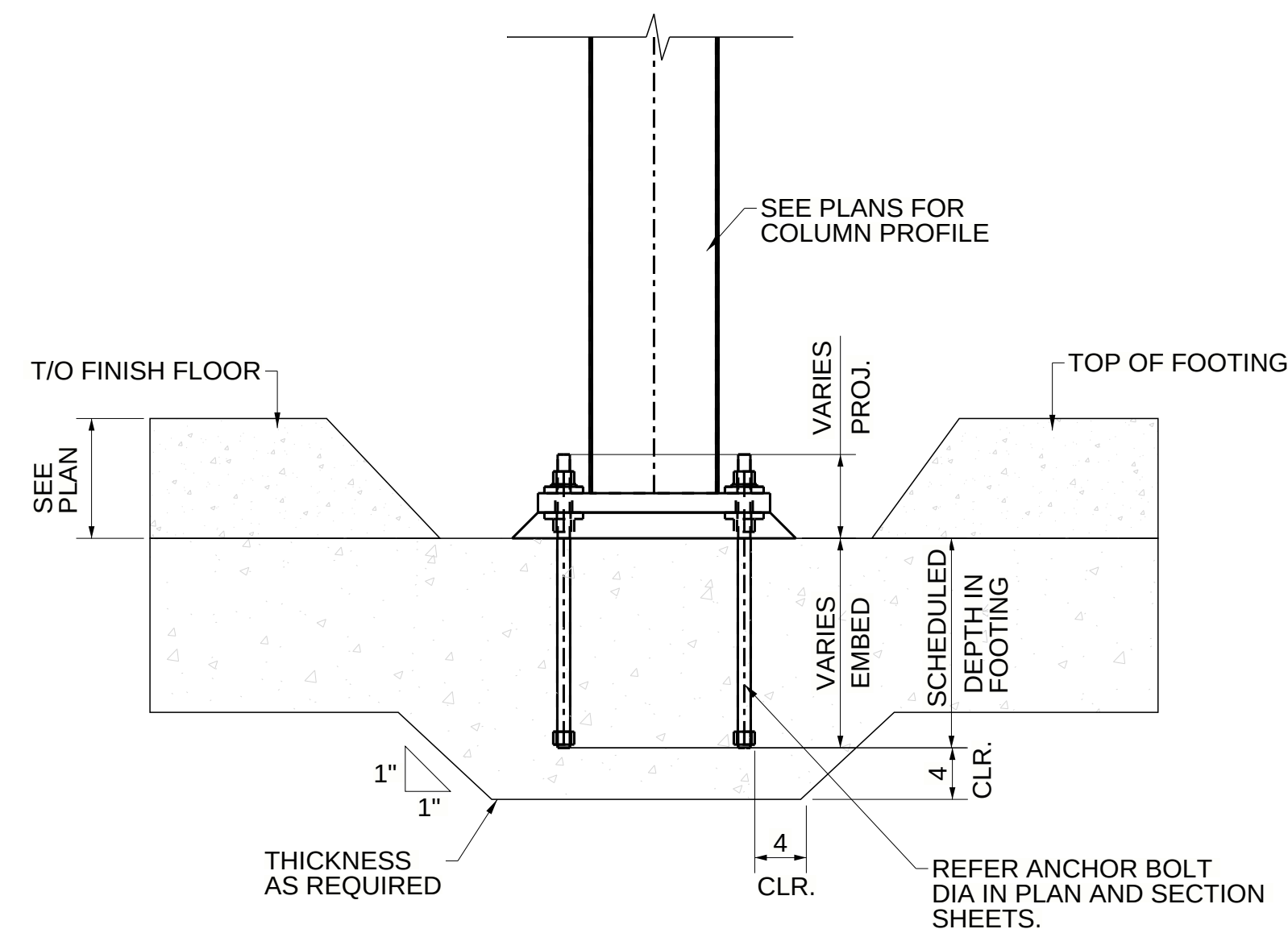
TYPICAL FOOTING DETAIL FOR DEPTH FOR EXCEEDING EMBEDS ( REFER : TYPICAL THICKEN FOOTING AT ANCHOR BOLTS 9 / S0.4 )
