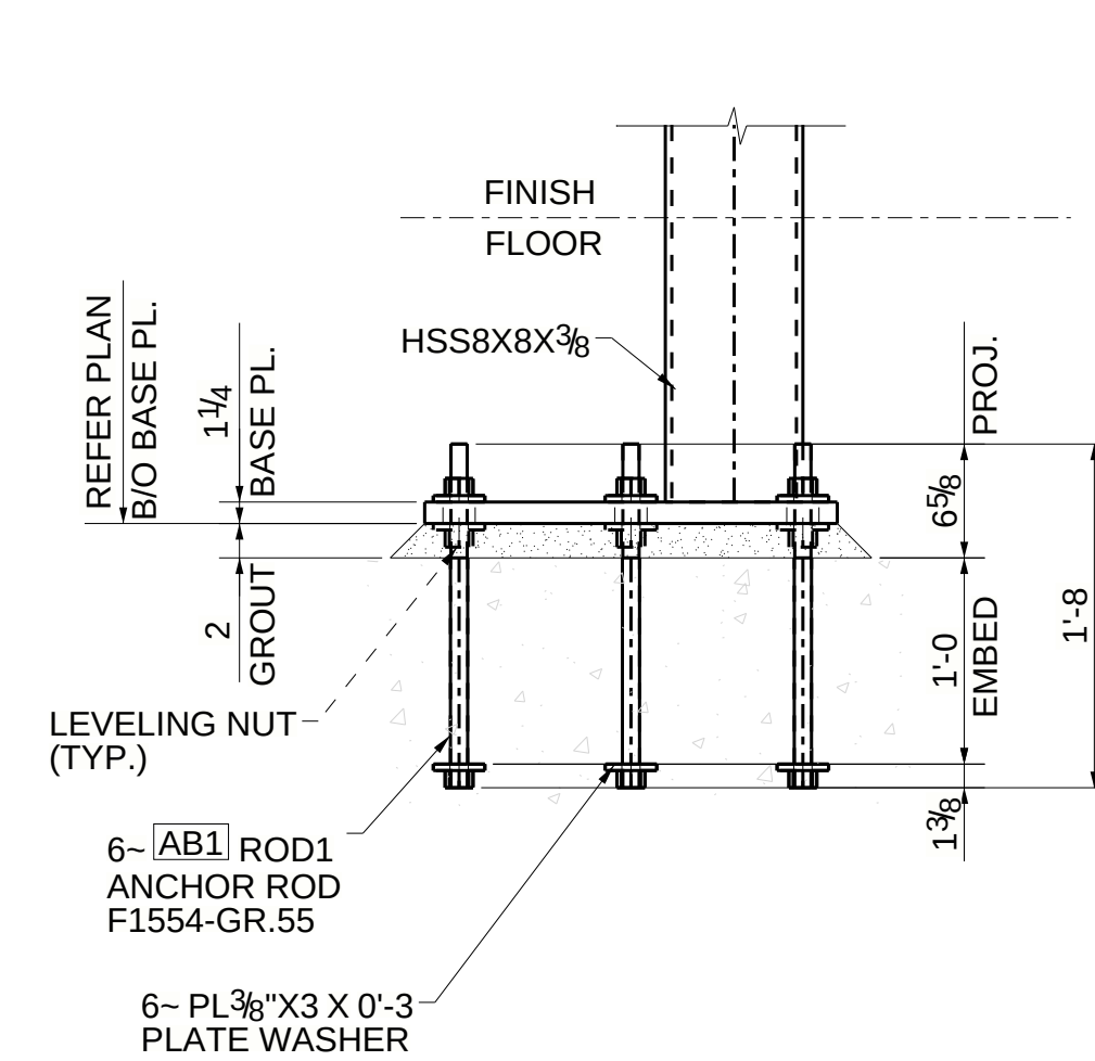
TYPE-4 (08 LOCATIONS)
