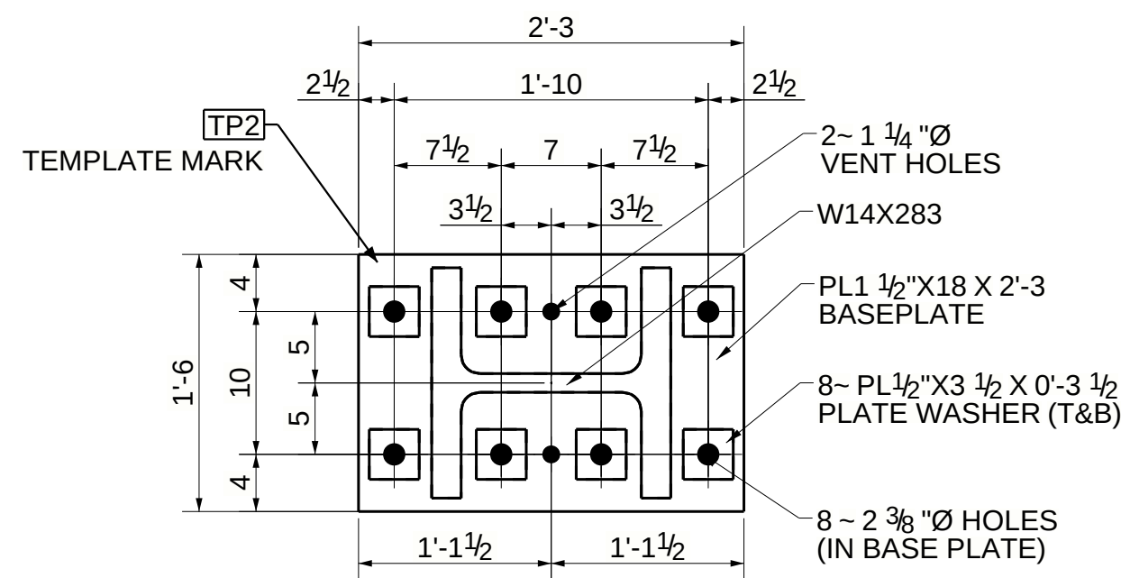
TYPE-2 (04 LOCATIONS)
