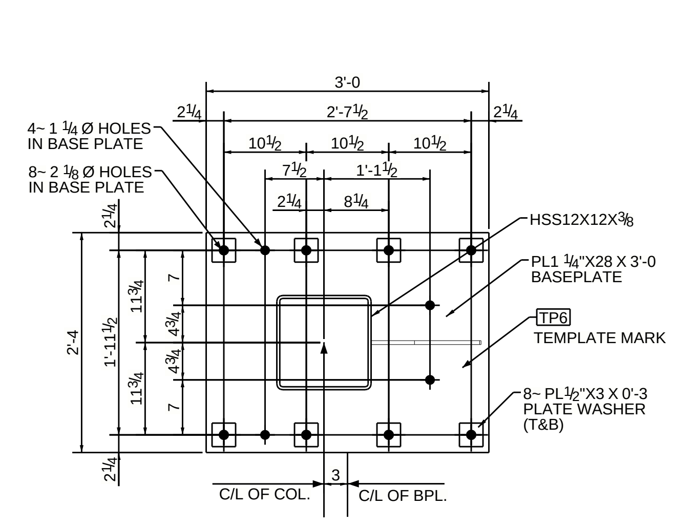
TYPE-8 (12-LOCATIONS) REFER PLAN FOR BASE PLATE ORIENTATION
