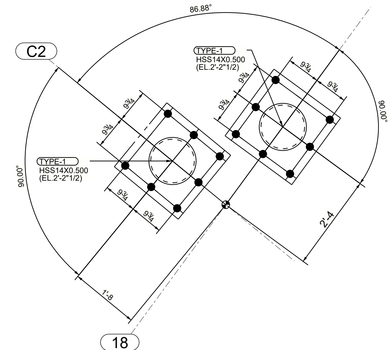
DETAIL D 1-A102
