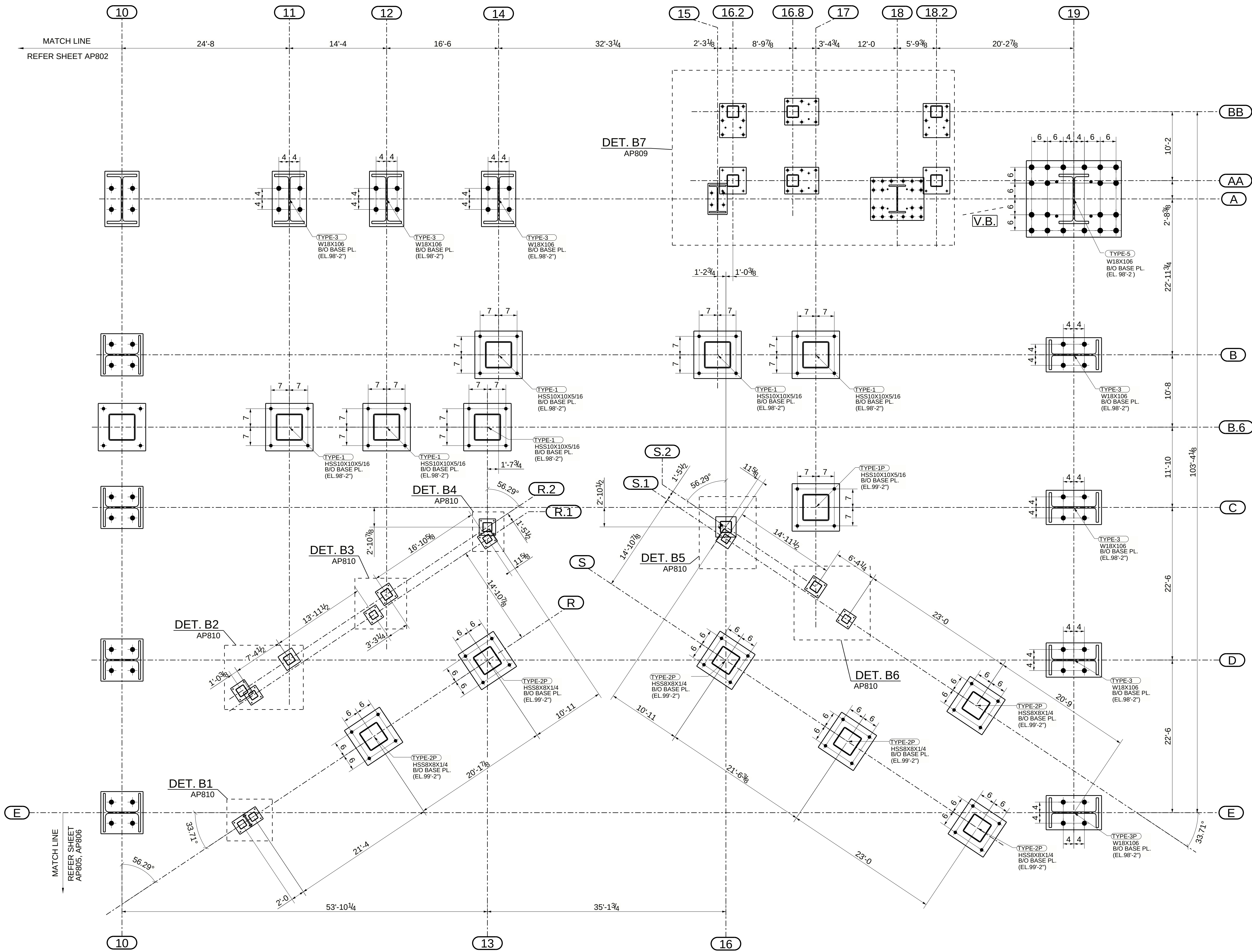
DETAIL B AP801 PARTIAL ANCHOR BOLT SETTING PLAN (REFER : OVERALL FOUNDATION AND SLAB PLAN 1/S - 100 & & PARTIAL FOUNDATION AND SLAB PLAN 1/ S-101& S-102)
