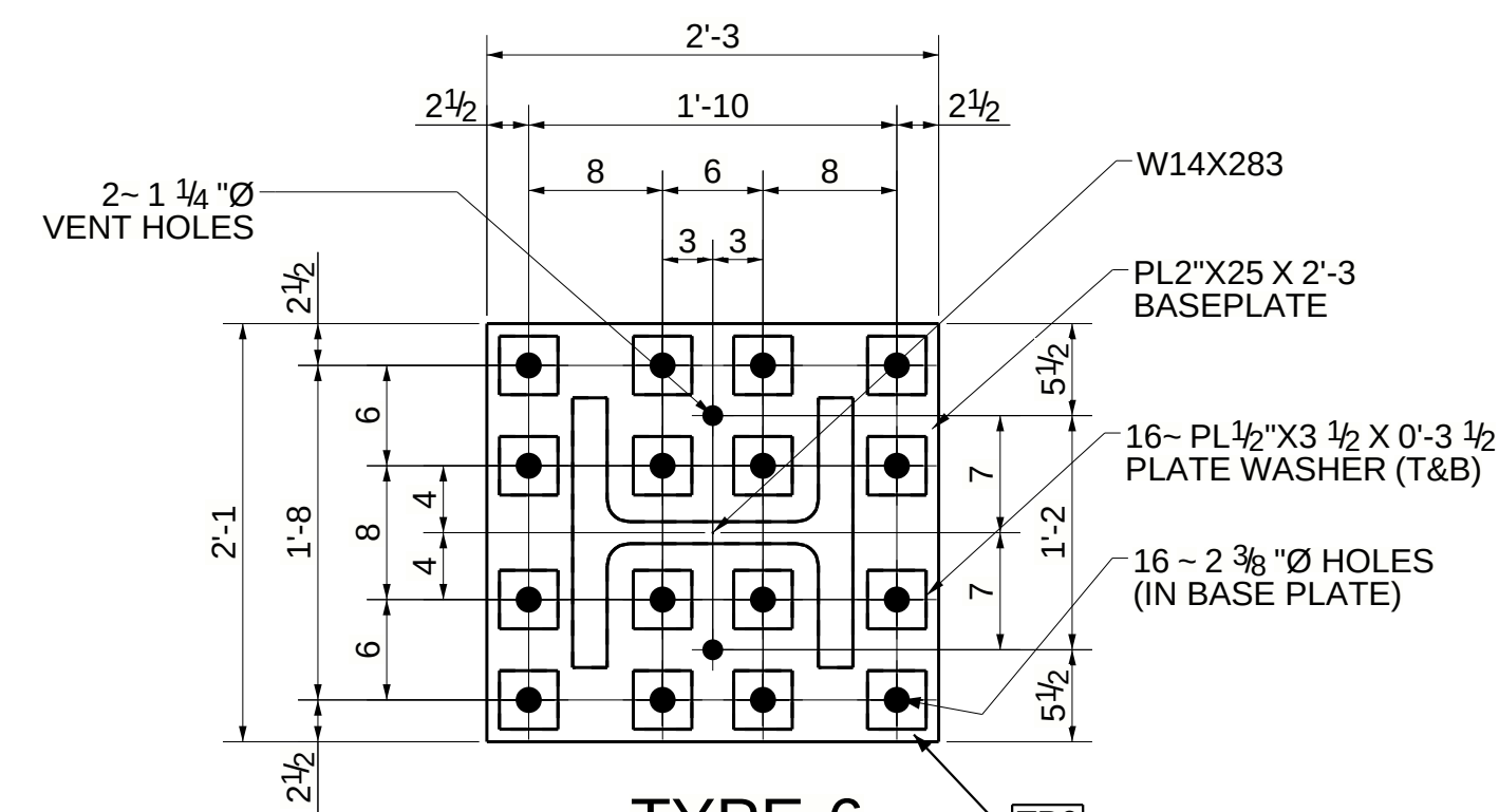
TYPE-6 (04 LOCATIONS)
