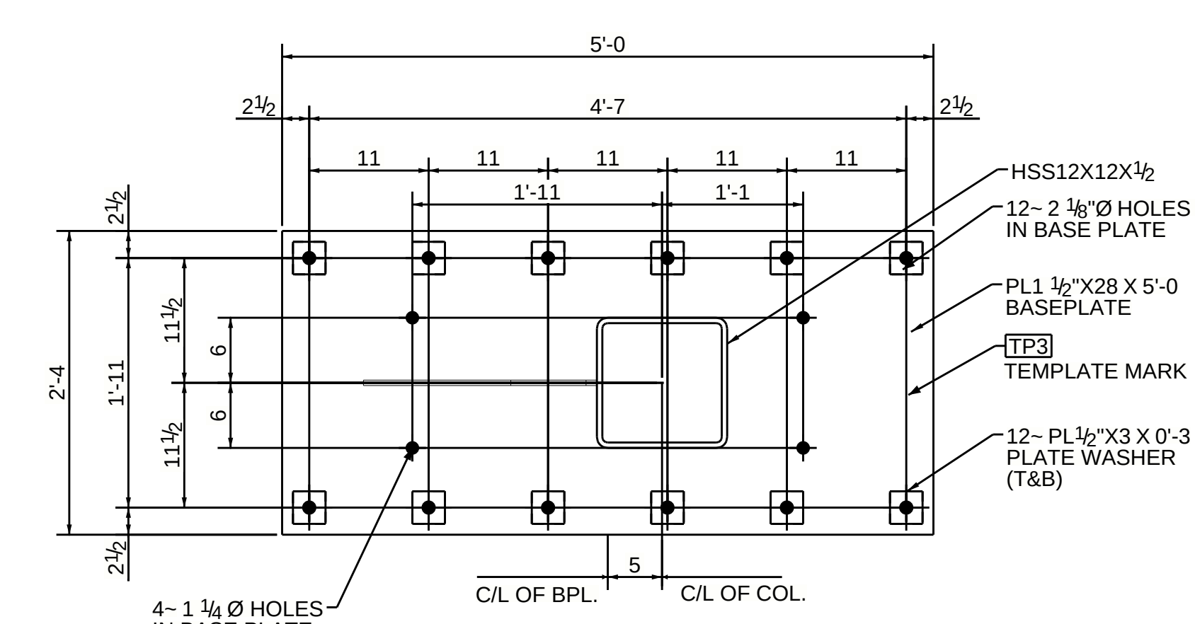
TYPE-3 (16-LOCATIONS) REFER PLAN FOR BASE PLATE ORIENTATION
