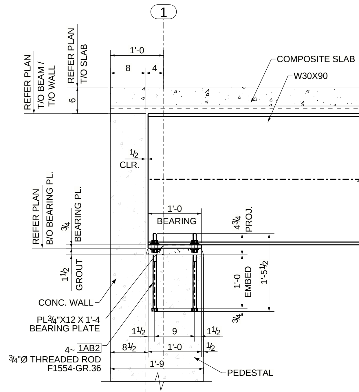
SECTION 5 - 5
