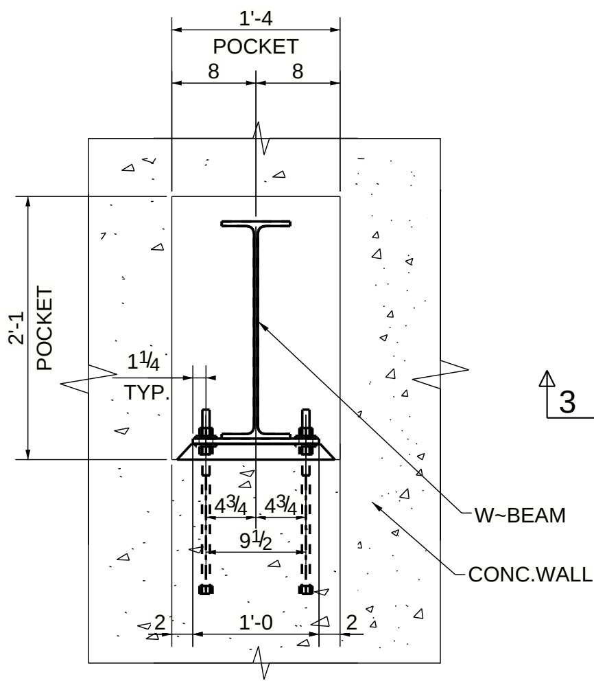
SECTION 2 - 2
