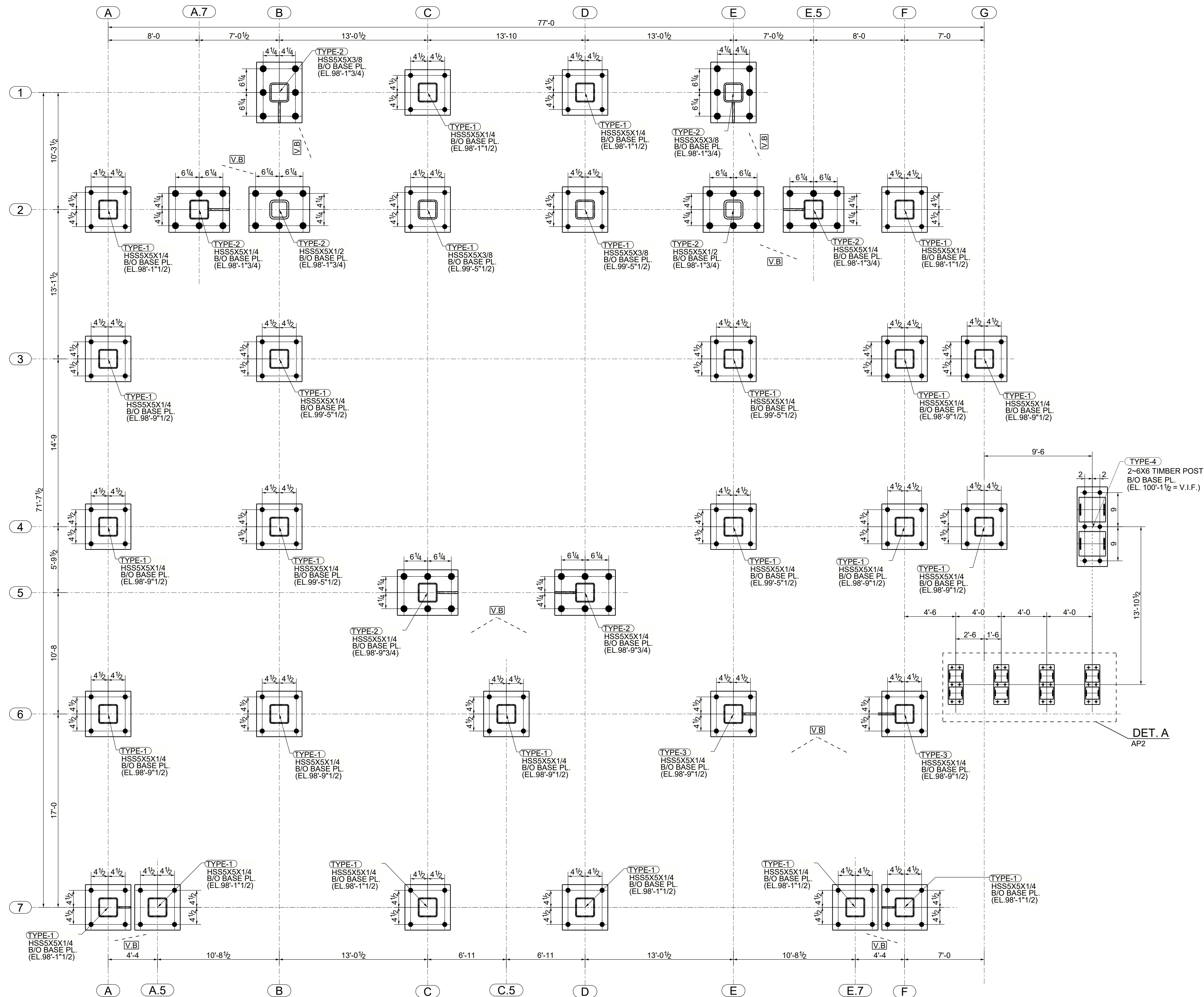
ANCHOR BOLT SETTING PLAN (REFER : FOUNDATION PLAN 1/S.1.1)
