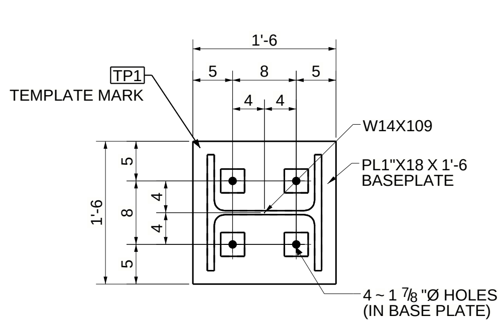
TYPE-1 (18 LOCATIONS)
