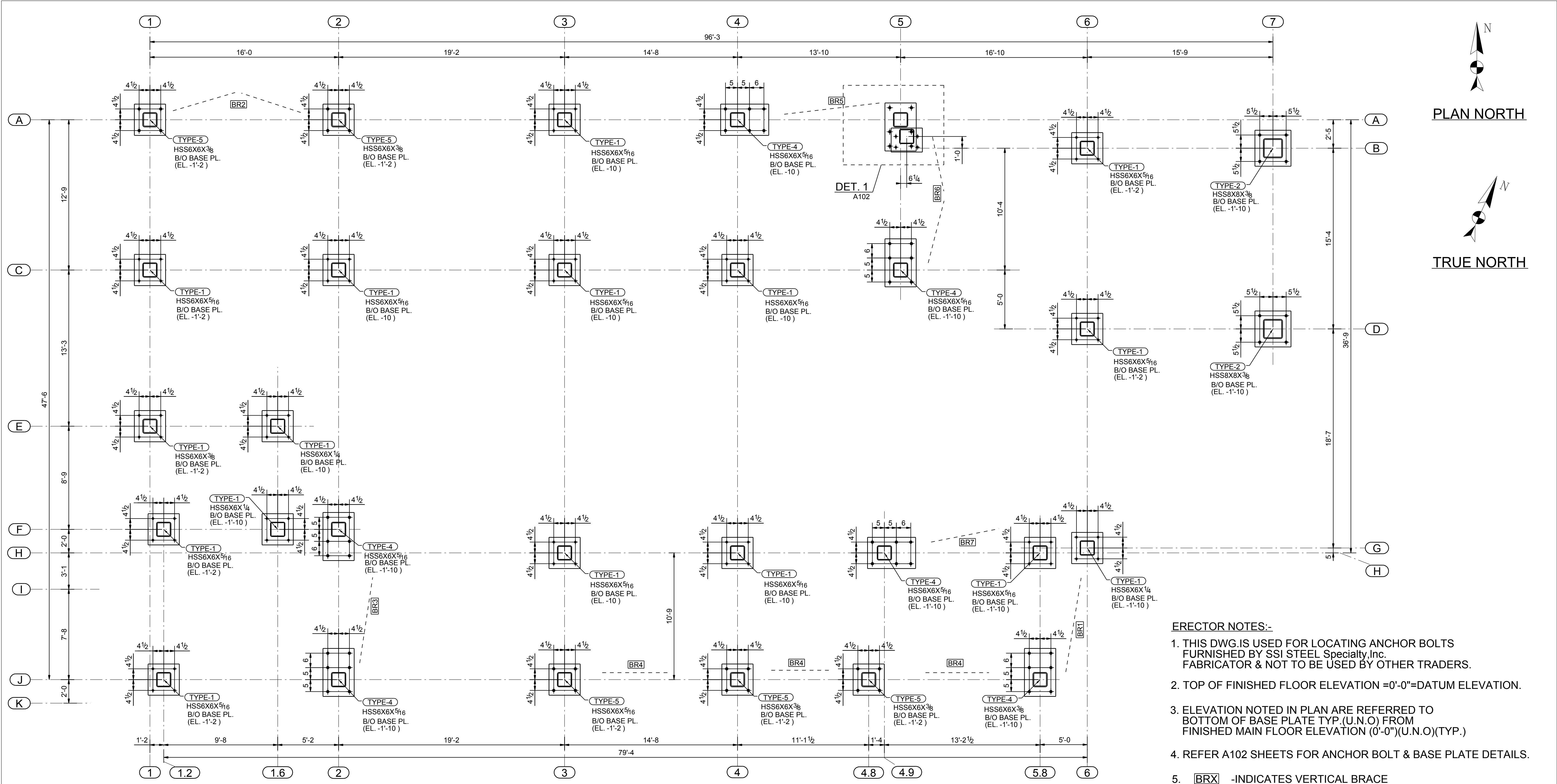
ANCHOR BOLT SETTING PLAN & GRID LOCATION PLAN (REFER : FOUNDATION + FLOOR SLAB PLAN 1/S1.01)
