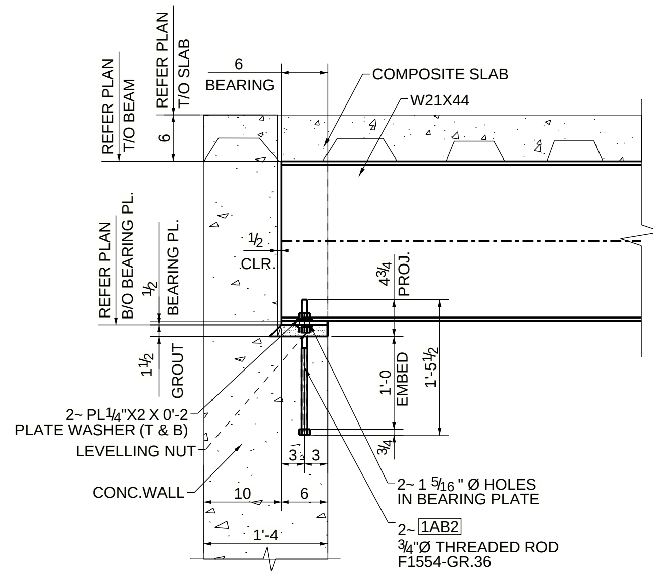
SECTION 1 - 1
