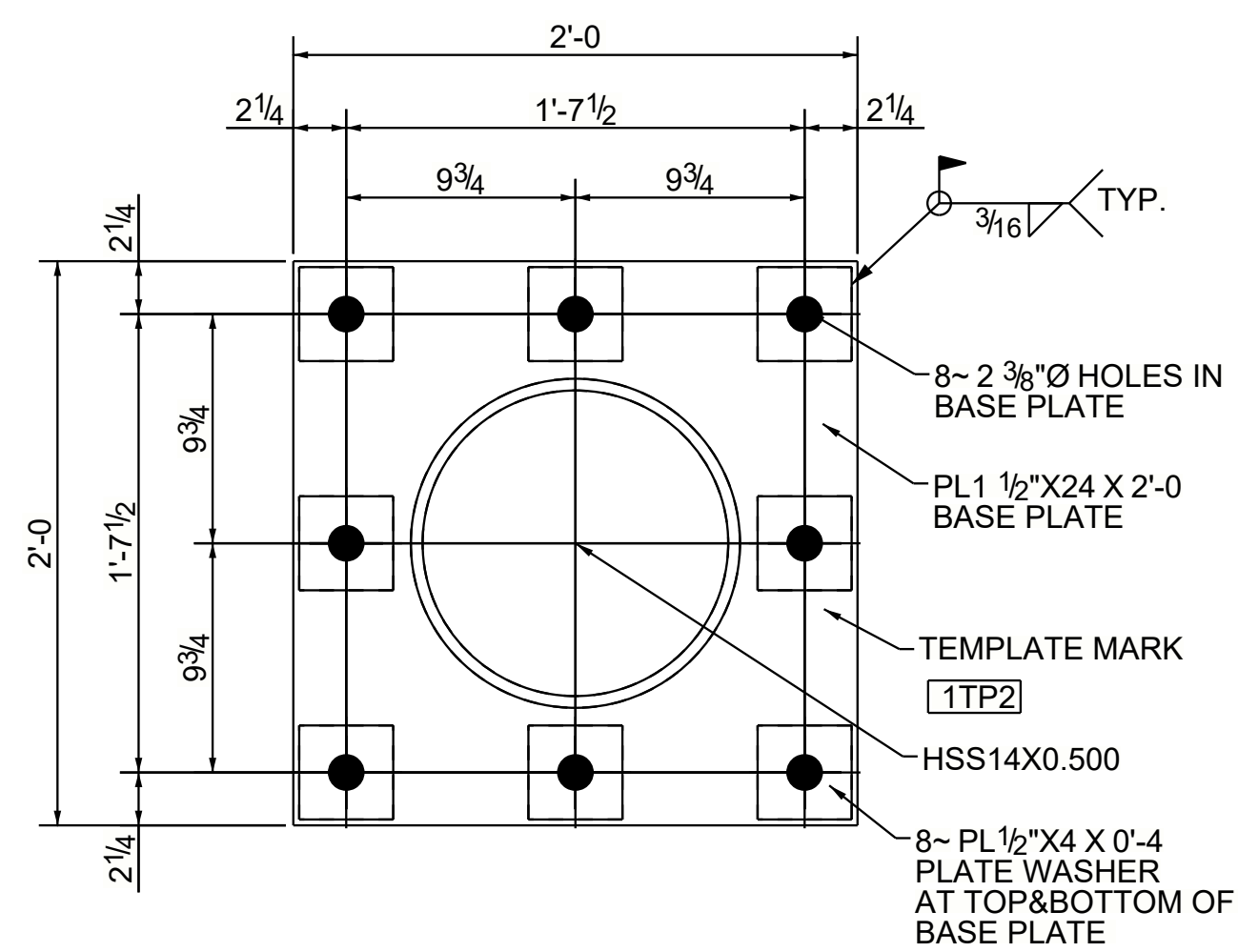
TYPE-1 (14-LOCATIONS)
