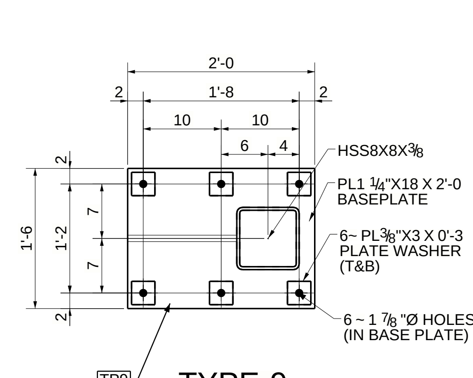
TYPE-9 (04 LOCATIONS)
