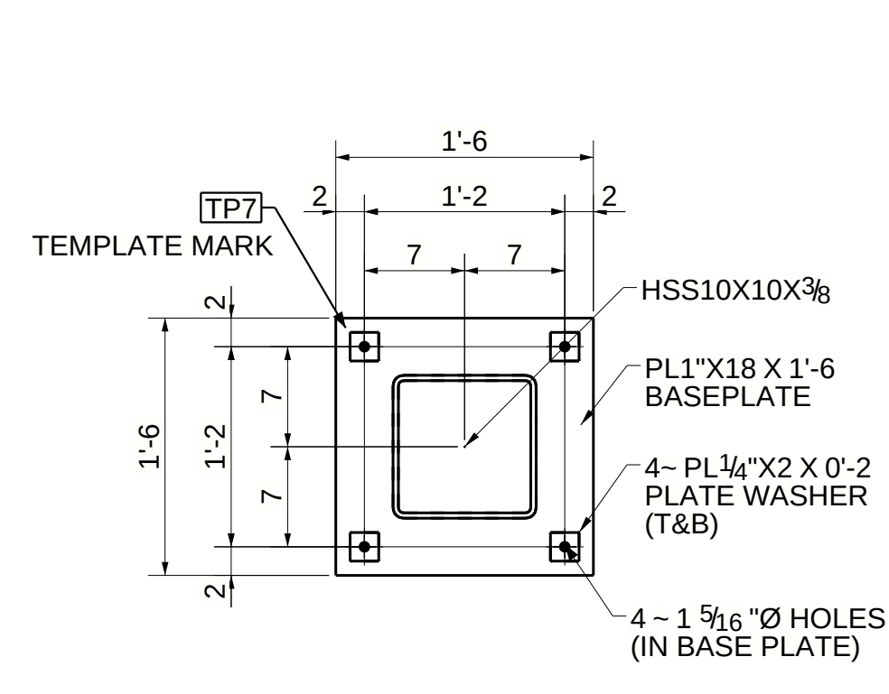
TYPE-7 (17 LOCATIONS)
