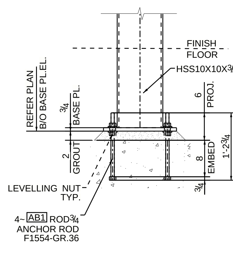
TYPE-3 (16-LOCATIONS) REFER PLAN FOR BASE PLATE ORIENTATION
