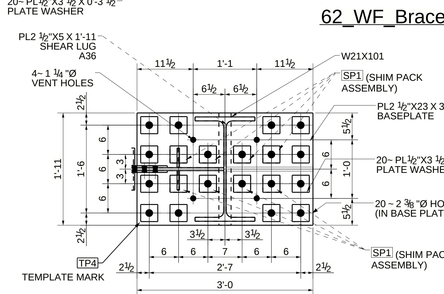
TYPE-4 (08 LOCATIONS)
