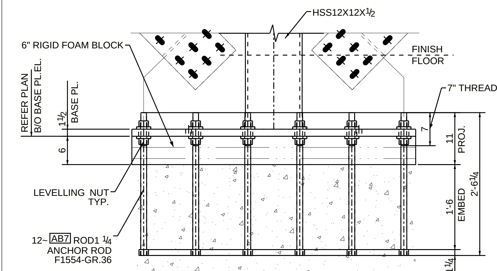
TYPE-1 (61-LOCATIONS) REFER PLAN FOR BASE PLATE ORIENTATION
