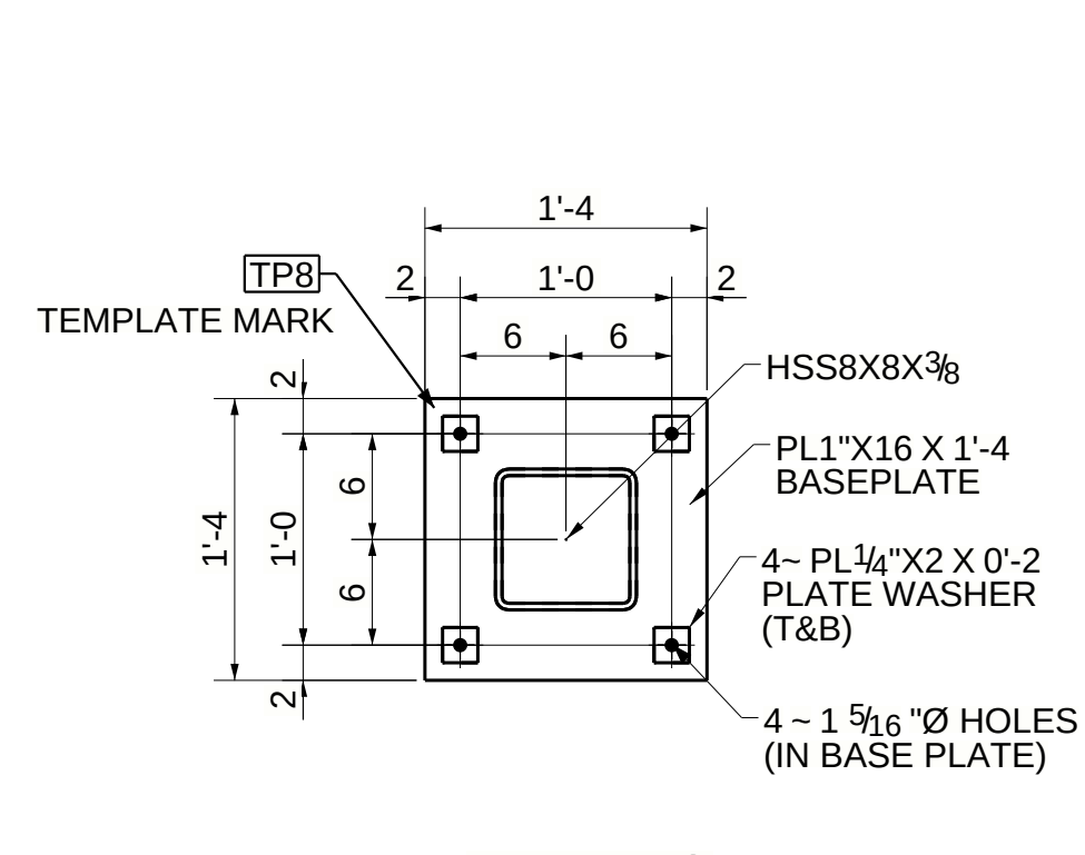
TYPE-8 (02 LOCATIONS)
