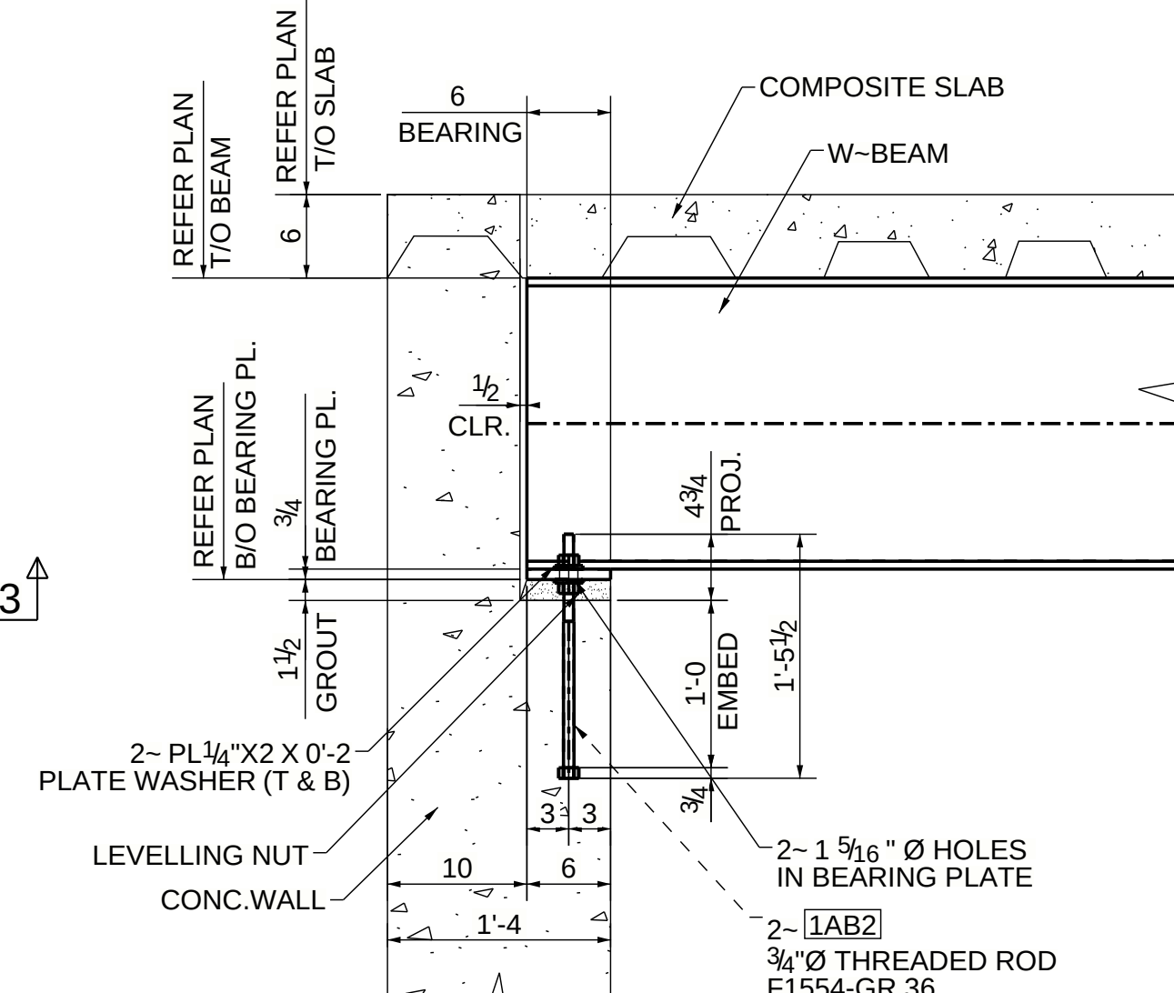
SECTION 3 - 3
