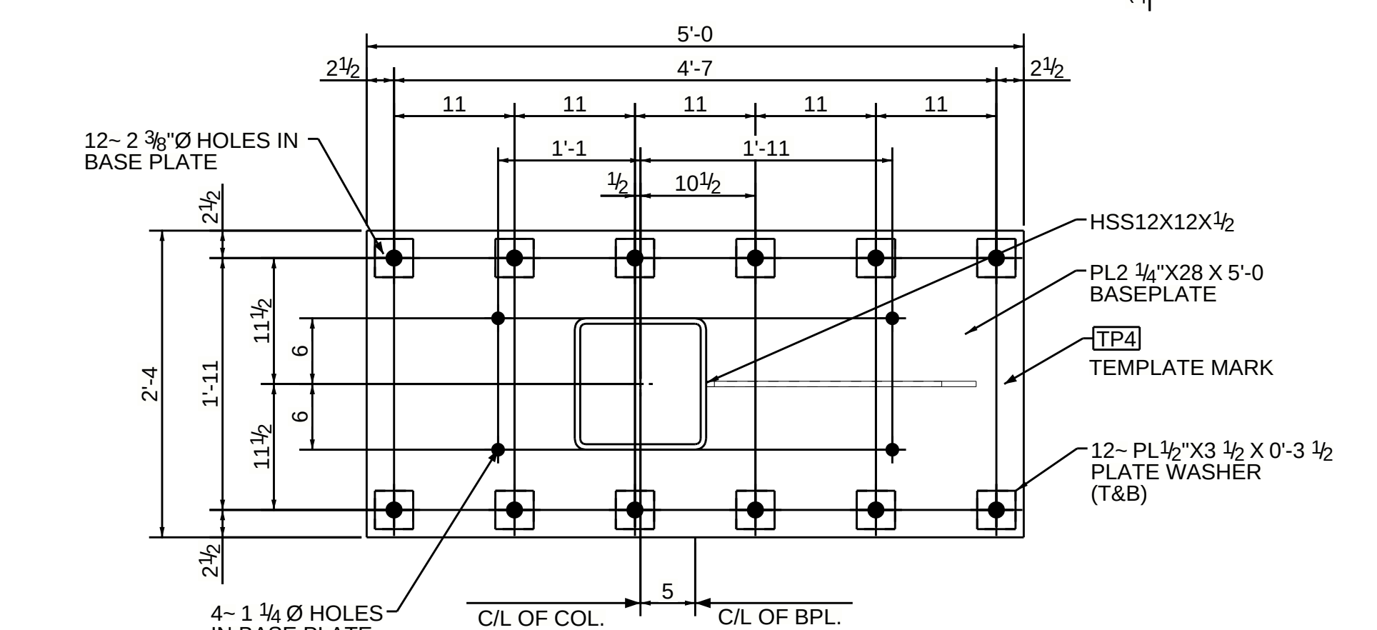
TYPE-4 (12-LOCATIONS) REFER PLAN FOR BASE PLATE ORIENTATION
