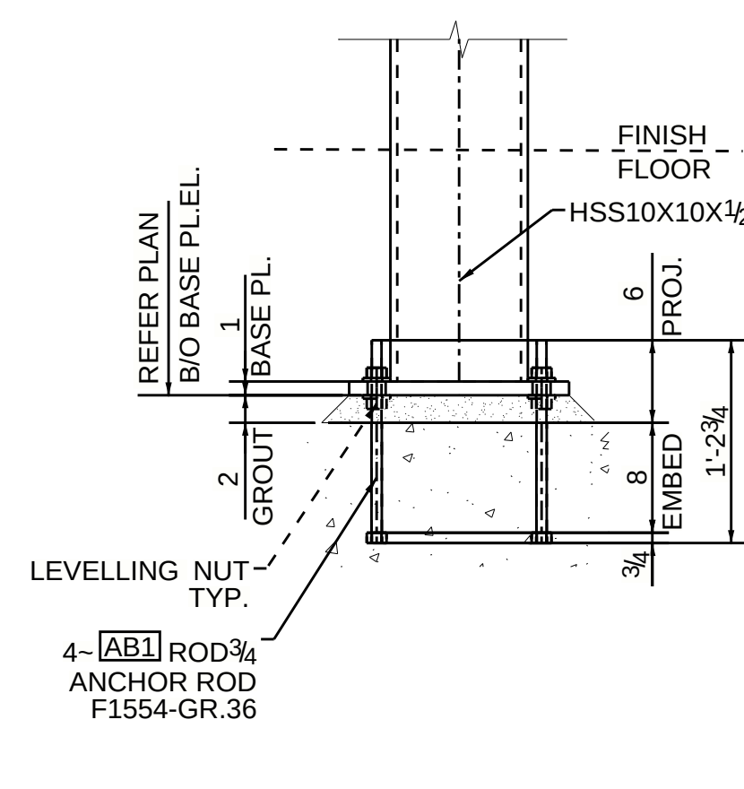
TYPE-2 (10-LOCATIONS) REFER PLAN FOR BASE PLATE ORIENTATION
