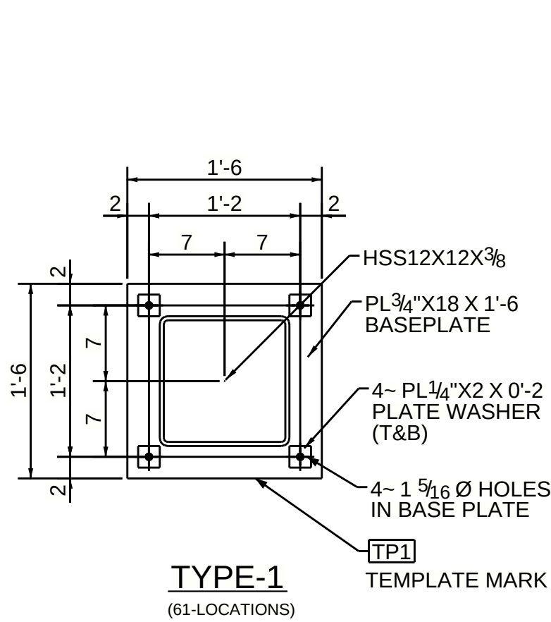
TYPE-1 (61-LOCATIONS) REFER PLAN FOR BASE PLATE ORIENTATION
