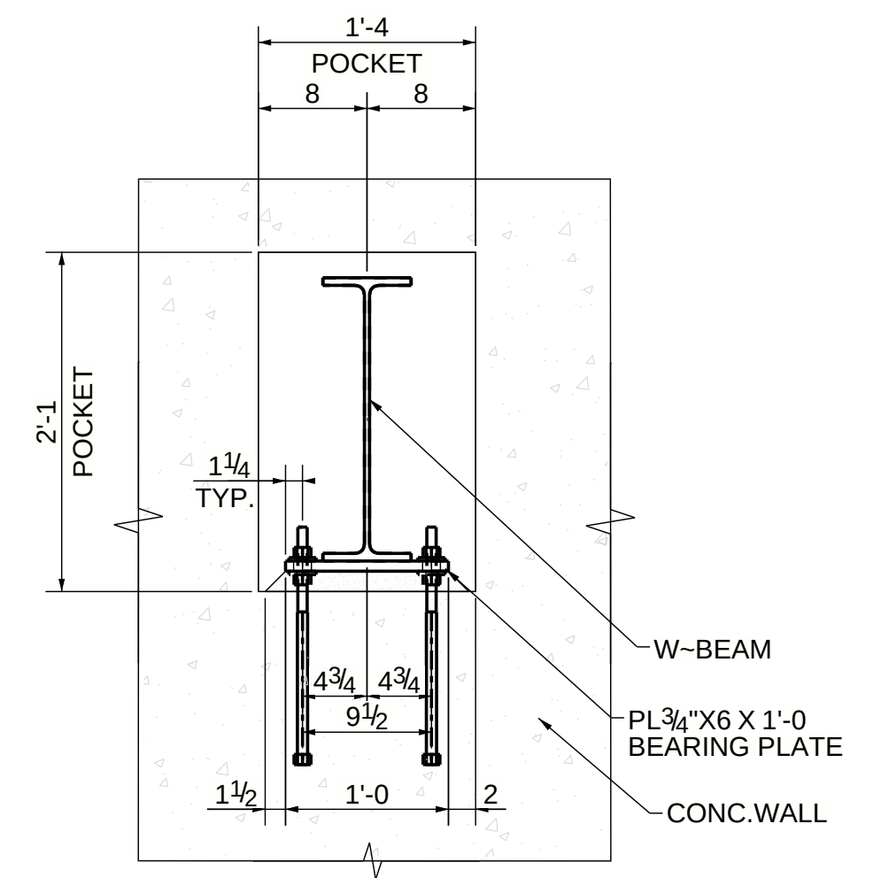
SECTION 4 - 4
